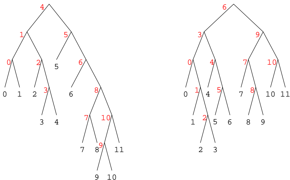
FIGURE 1. Tree pair diagram for x_0^2x_1x_2x_4x_5x_7x_8x_9^{-1}x_7^{-1}x_3^{-1}x_2^{-1}x_0^{-2} with carets and leaves numbered.
