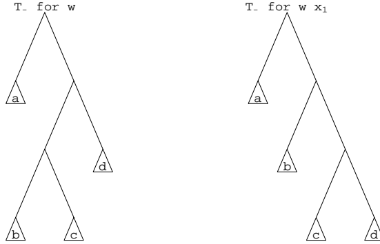
FIGURE 5. Right rotation around C_R induced by applying x_1
