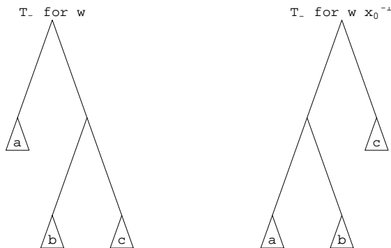
FIGURE 2. Rotation at the root induced by applying x_0^{-1} to T_- .
