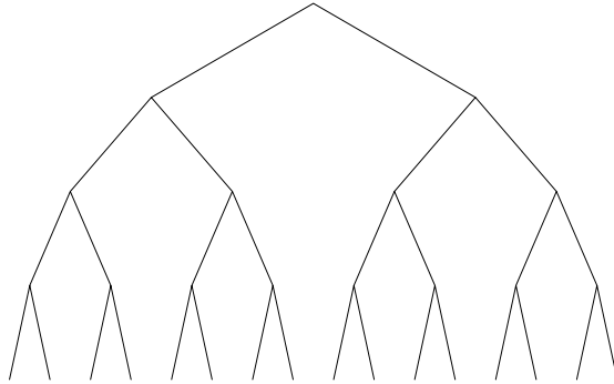
FIGURE 6. The balanced tree T_4
