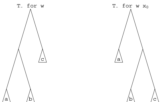
FIGURE 3. Rotation at the root induced by applying x_0 to T_- .
