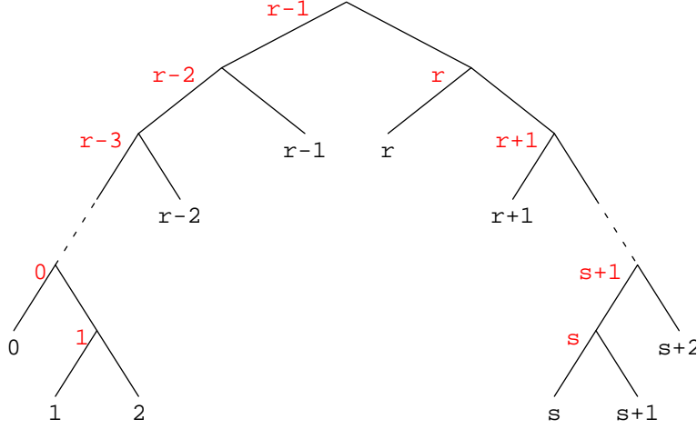
FIGURE 7. Positive tree for a word w \in \mathcal{C}(k)
