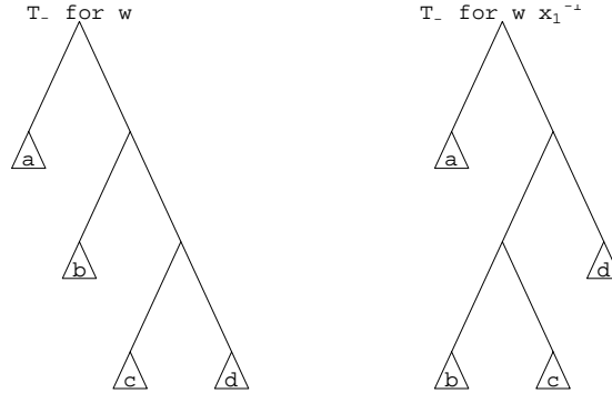
FIGURE 4. Left rotation around C_R induced by applying x_1^{-1}
