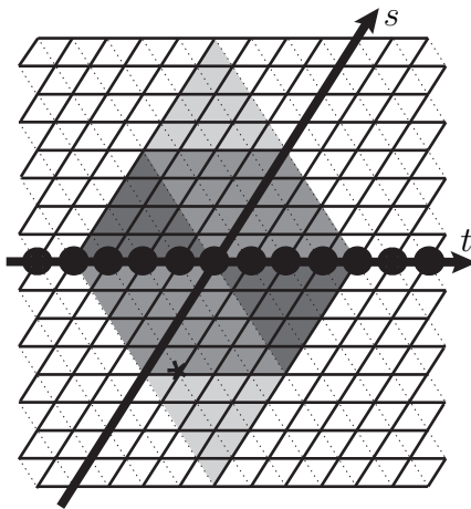
Figure 2: Diamond, hexagonal, and triangular regions in the lamplighting grid.
