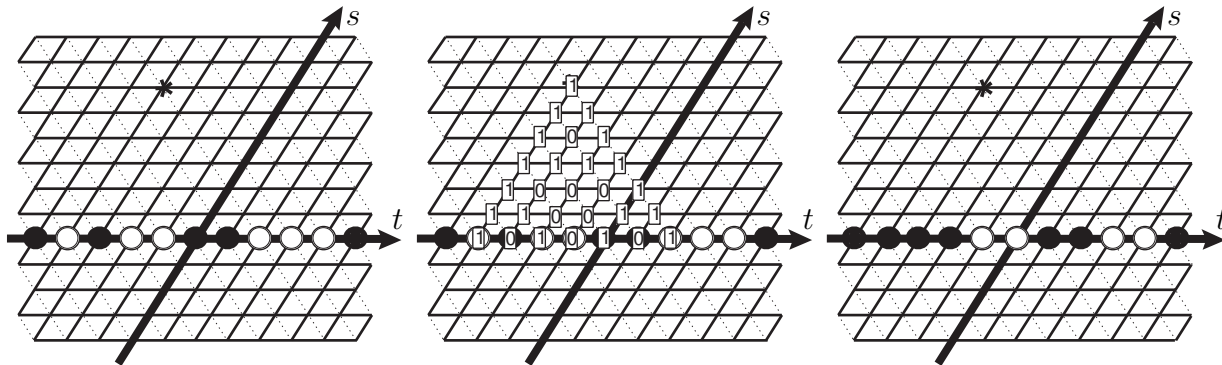
Figure 1: An example of the action of a . The left diagram shows g(\emptyset, (0, 0)) and the right diagram shows ag(\emptyset, (0, 0)) , where g = s^6at^{-2}at^{-1}at^{-3}at^{-1}at^{-1}at^4 . Along the t axis, open circles indicate illuminated lamps and filled-in circles indicate lamps which are off.
